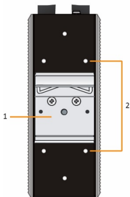
Rear Panel
