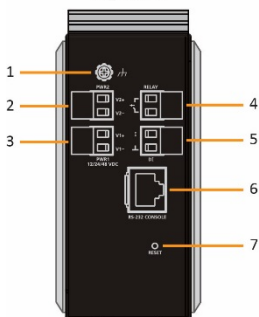
Rear Panel
