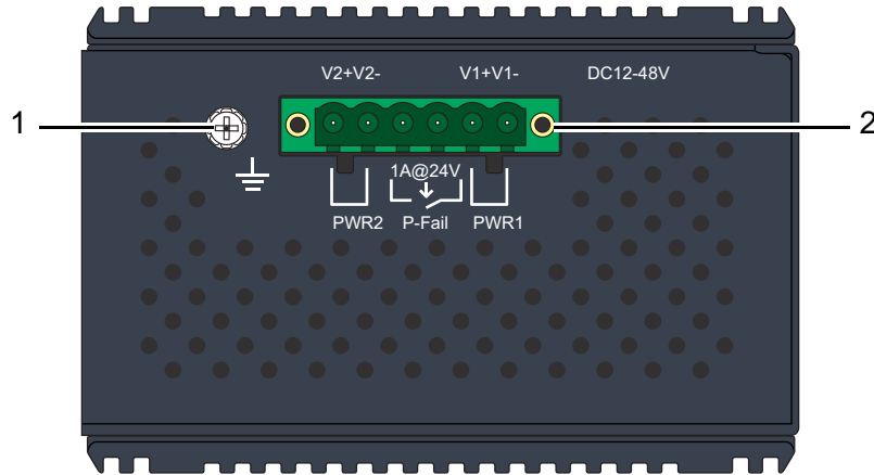
Figure 1.4 Top View
