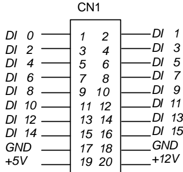
Figure 2.9.2 Pin Assignment of CN1
