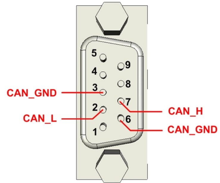
DB-37 to Male DB-9 Connector_CAN
